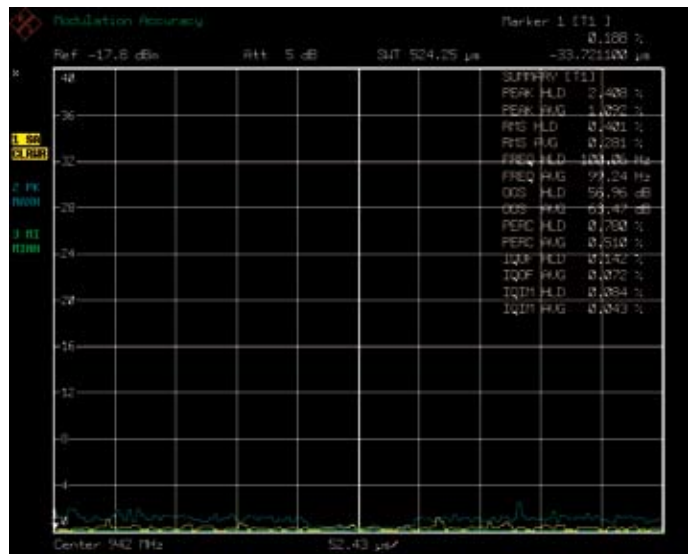
Measurement of modulation accuracy on EDGE burst.
