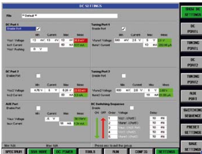
Menu for setting the DC ports for signal source analysis and additional port for negative supply voltage.
